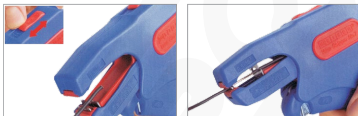
Stripped insulation thickness adjustment
