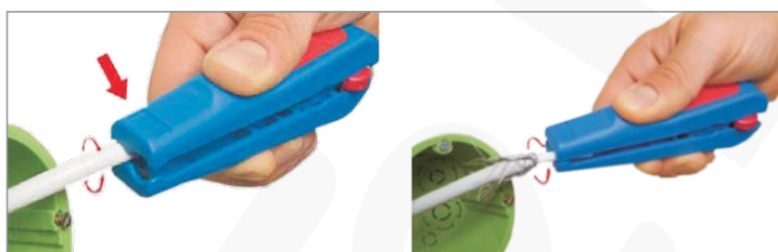
Stripping external insulation
