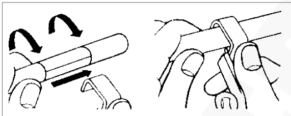
Stripping insulation from the middle of cable
